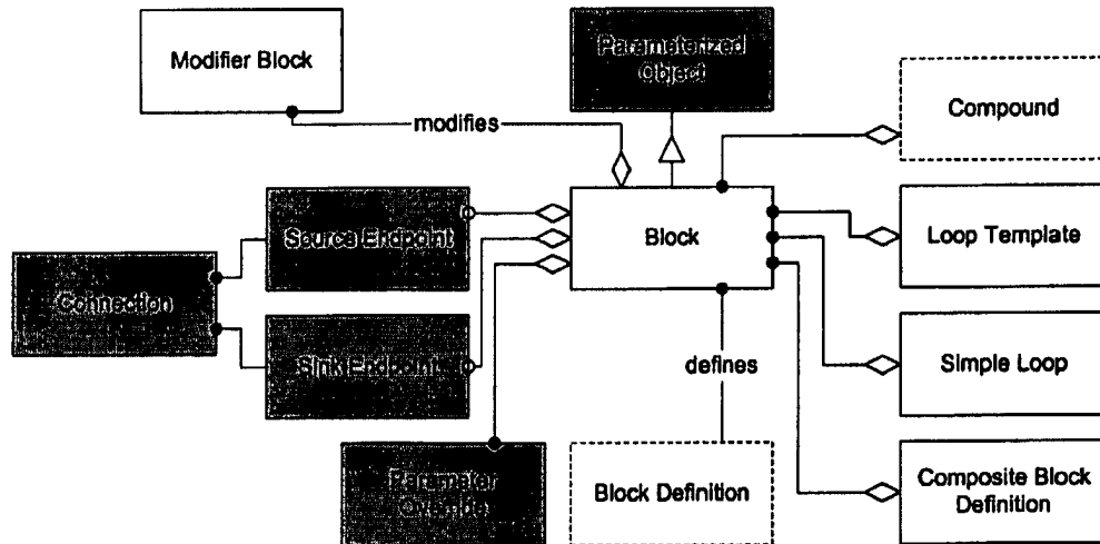
Figure 84 - Block object model
